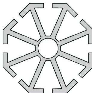
40x40 ALU-8 with 8 rails in 45 degree angles. Excellent as singel standing foot with multi functions. M10 thread in one or both ends. Black powder coating available.
